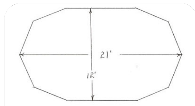
GAZEBO DIMENSIONS:
